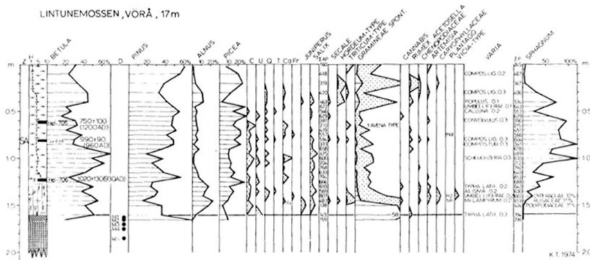
Fig. 23. Pollen diagram from profile Vöyri I.
