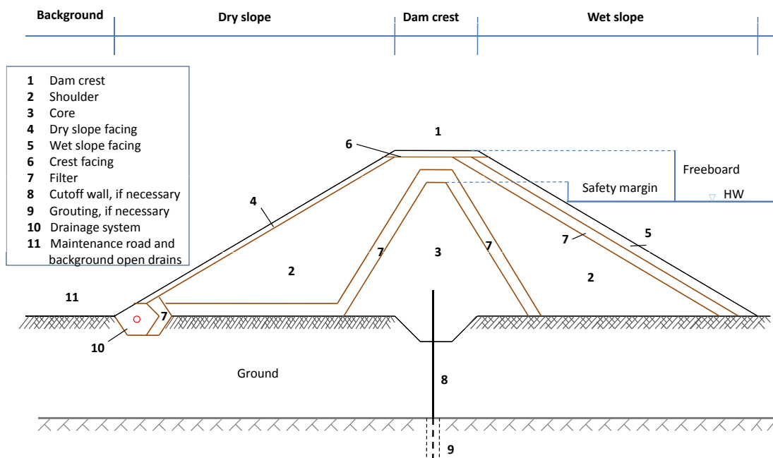
Figure 1. Cross-section of an embankment dam and its structural parts.
