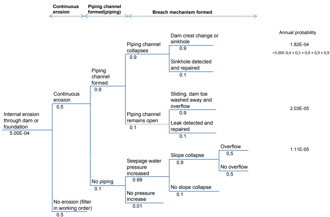
Figure 2. Example of an internal erosion event tree analysis.
