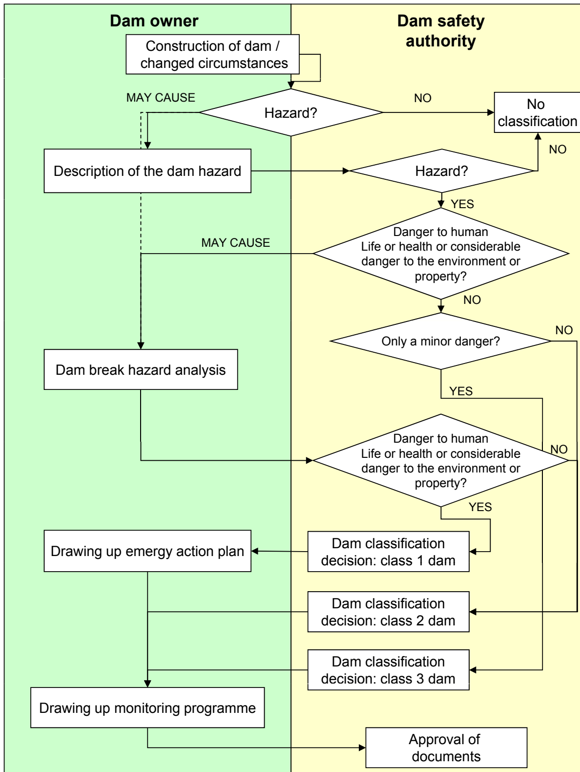
Figure 3. Dam classification and document approval.
