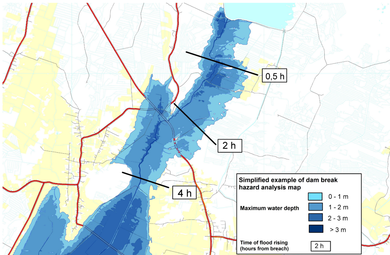
Figure 1. Example of a dam break hazard analysis presentation (Map: Mikko Huokuna, 2010).
