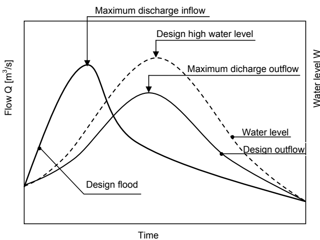
Figure 1. An example of design flood, design outflow and water level in the reservoir, (Figure: Pekka Vuola, 2006).
