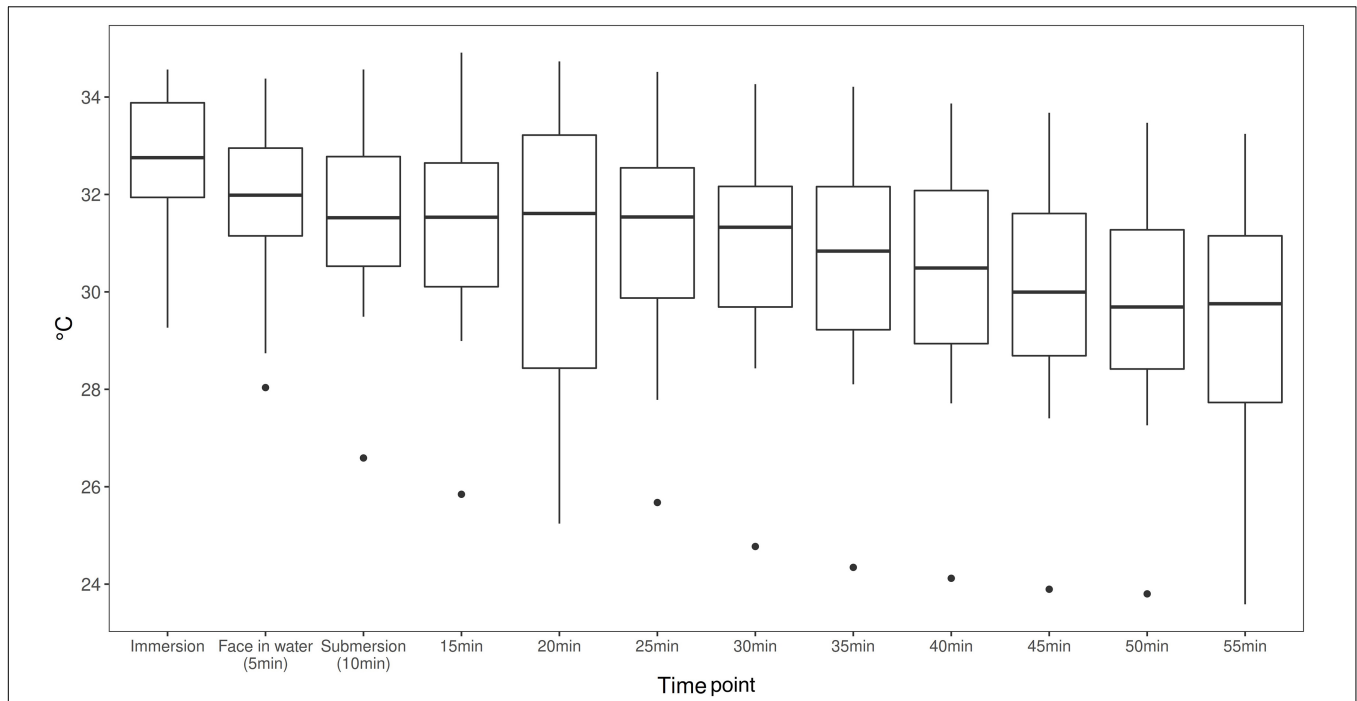
FIGURE 3 | Area weighted skin temperature ( T_{skin} ) calculated from the four skin temperature measures with standardized weighting coefficients at a 5-min interval during the dives ( T_{skin} = neck*0.28 + scapula*0.28 + hand*0.16 + shin*0.28 ) [ISO 15027-3:2012(E)]. Means and range shown ( n = 26 ).
