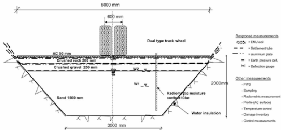
Cross section and instrumentation of the structure
