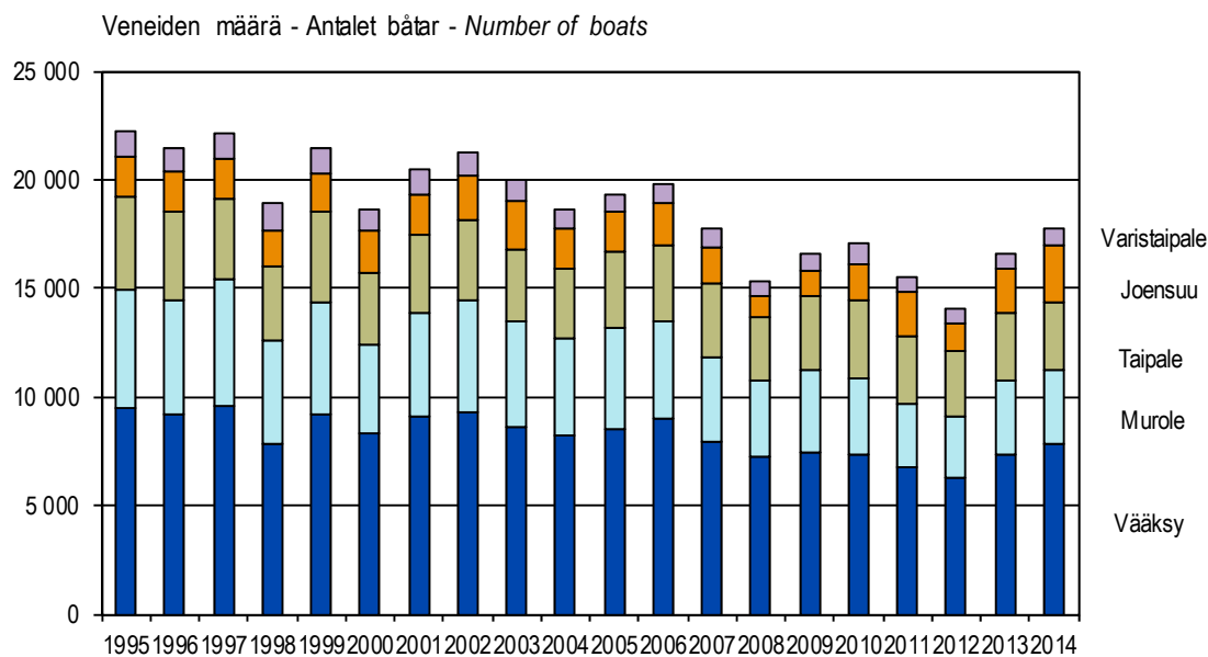
Figure 13. Number of lockages of pleasure crafts by five service lock canals, 1995-2014
